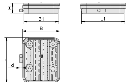
VCBL-G-K1 140x115
